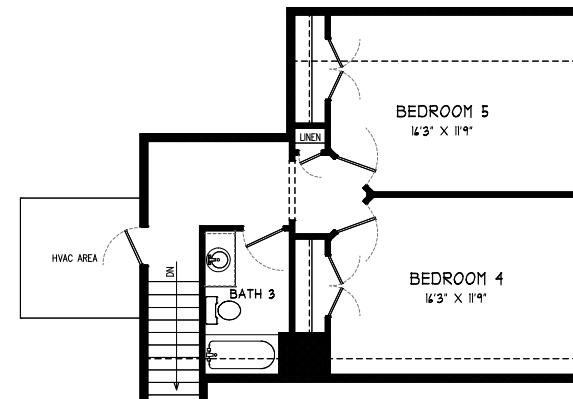
OPTIONAL SECOND FLOOR PLAN
