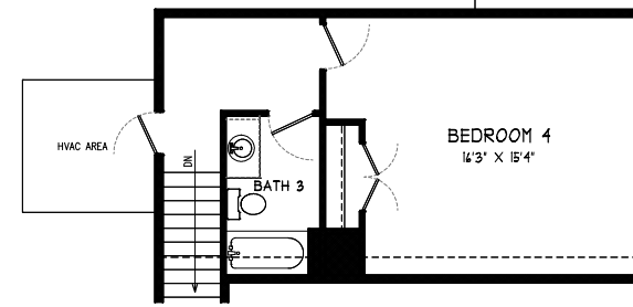
OPTIONAL SECOND FLOOR PLAN
