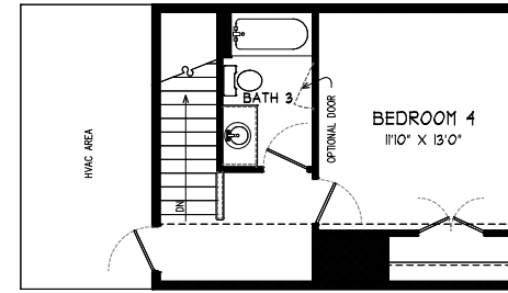
OPTIONAL SECOND FLOOR PLAN
