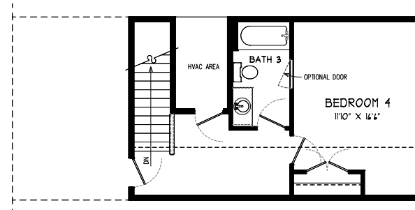
OPTIONAL SECOND FLOOR PLAN
